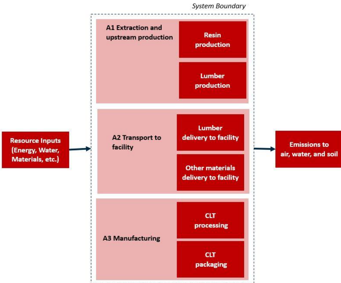
Figure 2: Cradle-to-Grave CLT Product System
